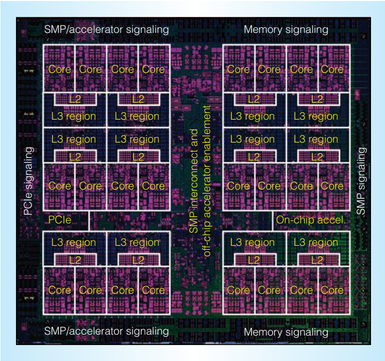
Figure 1. The Power9 chip diagram shows the number of cores, L2 and L3 cache regions, and interconnects.
