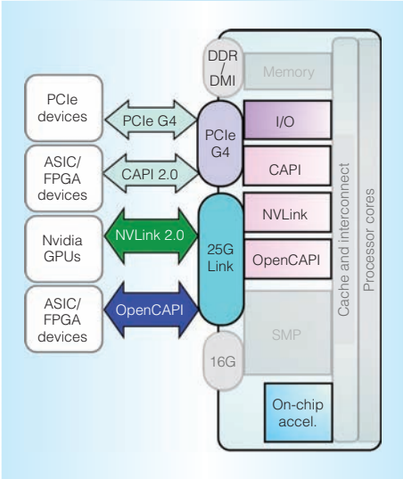
Figure 2. Power9 processor integration with external accelerating devices supporting PCIe Gen4, CAPI 2.0, NVLink2.0, and OpenCAPI.
