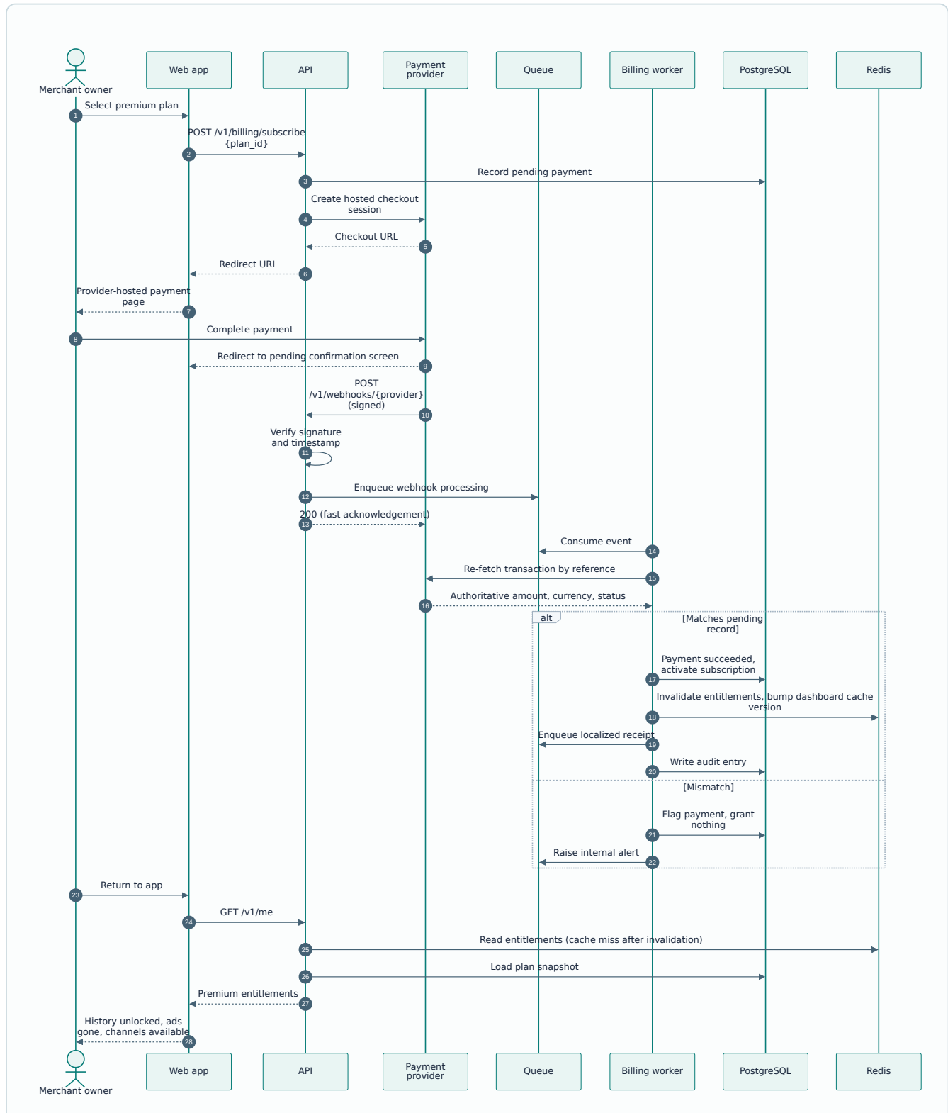
FIGURE 8 6.7 Sequence diagram — premium subscription activation
