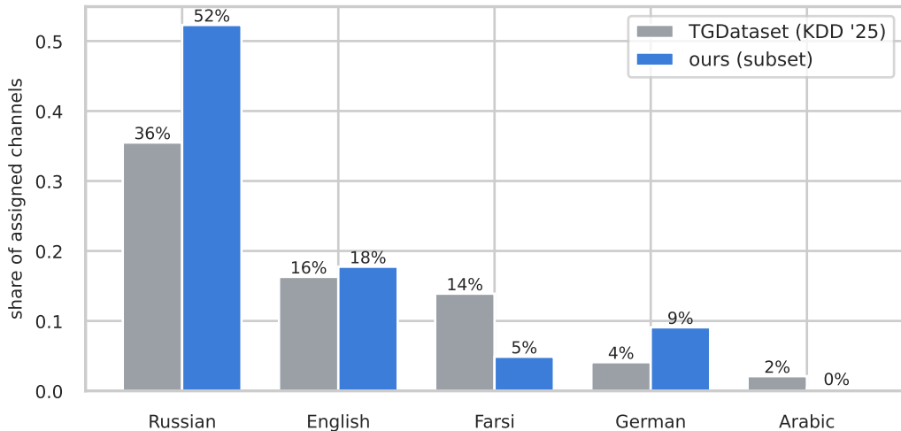
Channel-language distribution: ours vs TGDataset (>50% rule)
