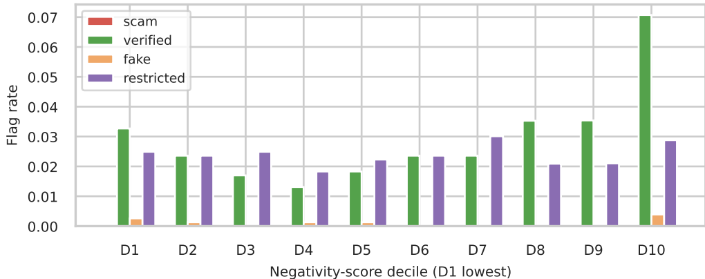
Telegram flag rates by reaction-negativity decile
