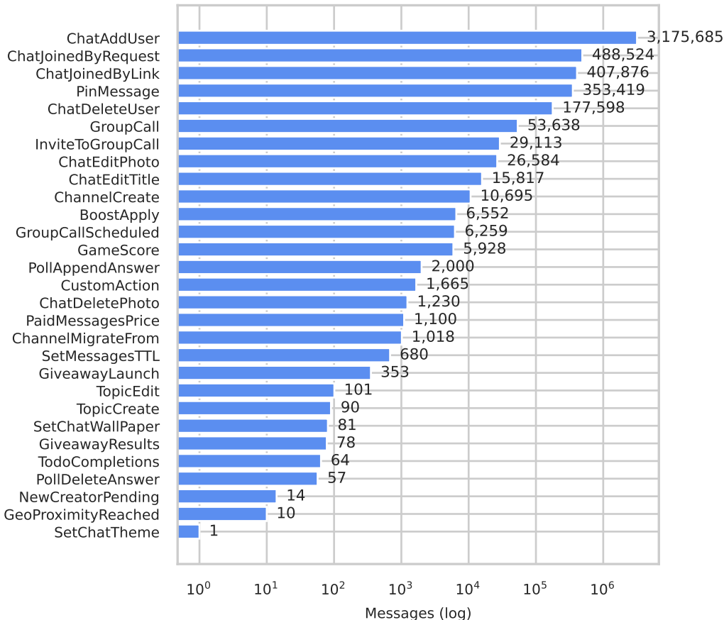
Service-action breakdown: 4,766,230 messages (as-of 2026-06-15)
