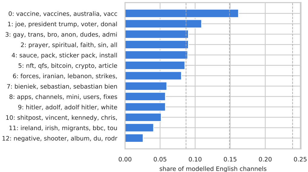
BERTopic topics over English channels (n=1,007): ours
