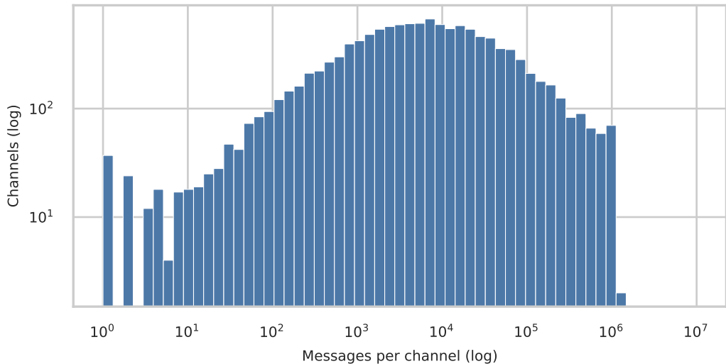
Per-channel message-count distribution (N = 12,065 channels with \geq 1 message)
