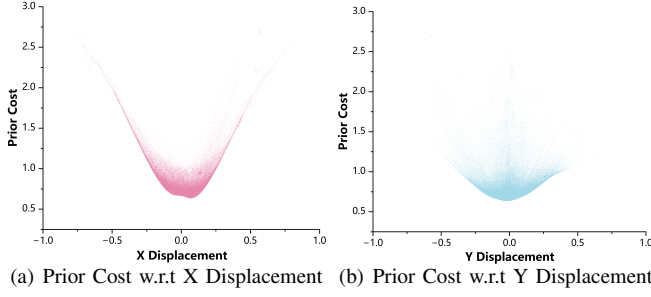
Fig. 7. Relationship between the prior cost and the displacement. Each point denotes a matching pair. The pedestrian displacements are separately shown along the (a) x -axis and (b) y -axis. The prior cost is generally positively correlated to the absolute value of displacement in both x and y direction, while the trends differ that the prior cost increase faster when pedestrians in frames move horizontally than move vertically.
