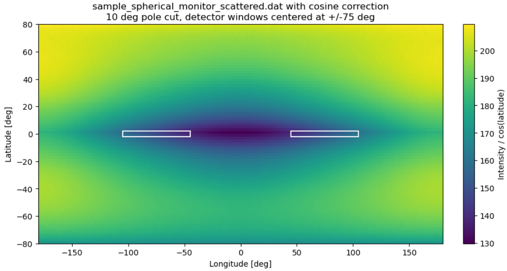
Figure 4.2: The heatmap obtained when simulating the vanadium sample in the CAMEA instrument. The white boxes are the equatorial latitude bands used later.
