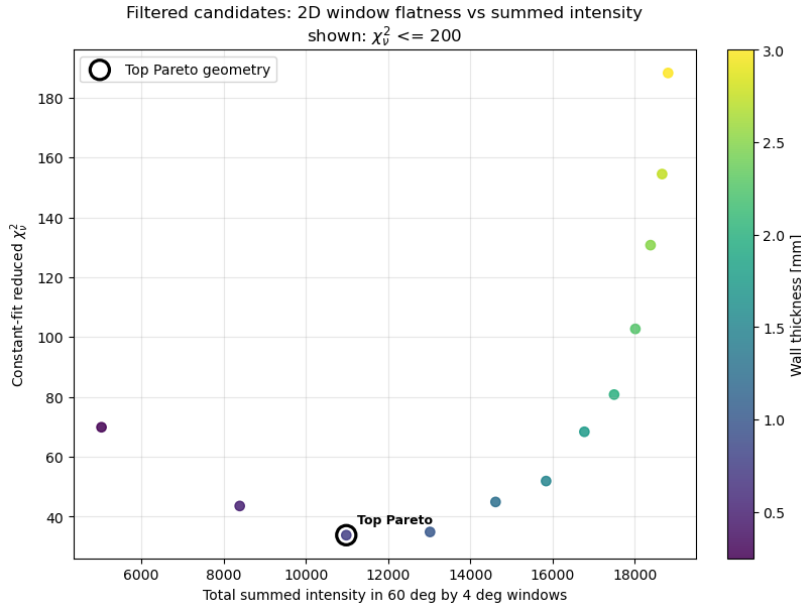
Figure 4.7: Pareto optimization with a sample of fixed height and radius.
