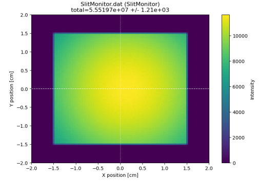
(b) Incoming beam profile from slit monitor intensity distribution.
