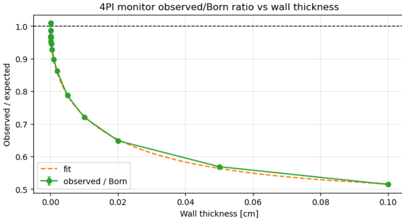
(a) Observed intensity over expected intensity as a function of wall thickness.
