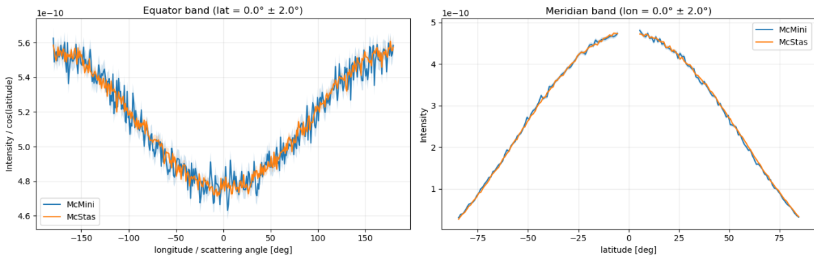
Figure 3.3: Equator and meridian cut for the solid cylinder case
