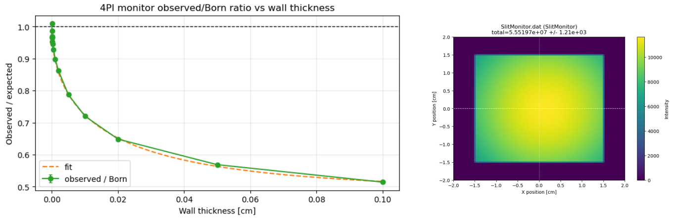
(a) Observed intensity over expected intensity as a function of wall thickness. (b) Incoming beam profile from slit monitor intensity distribution.
