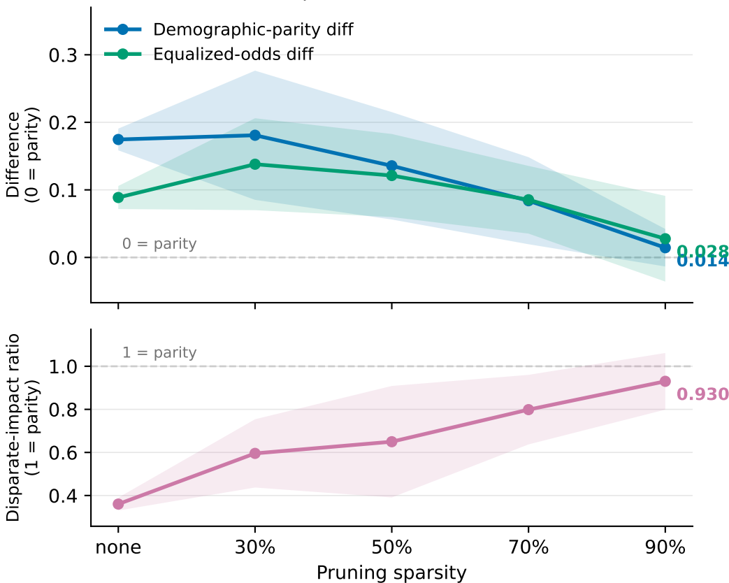
The fairness win depends on the metric (Adult MLP, sex)
