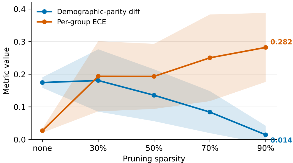
Compression hides unfairness (Adult MLP, sex)
