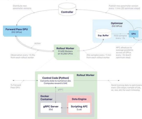
OpenAI Five paper: distributed training architecture
