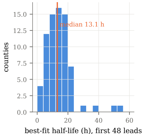
(b) per-county restoration half-life
