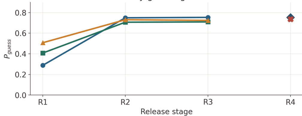
Identity-guessing success
