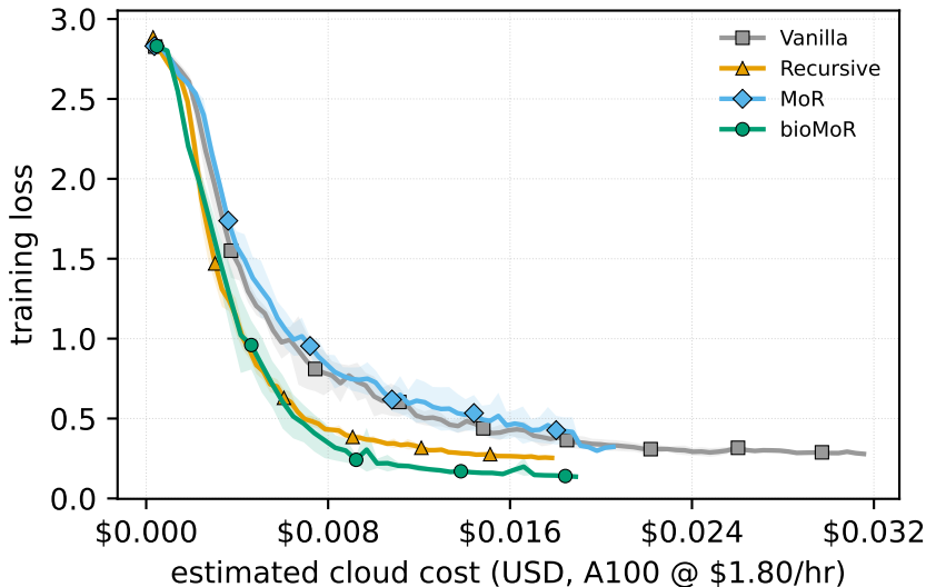
Baron (pancreas): training loss vs cost (5-fold CV)
