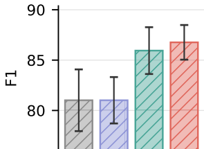
Pan-cancer (mutation+CNV)
