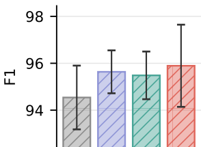
Pan-cancer (tri-modal)
