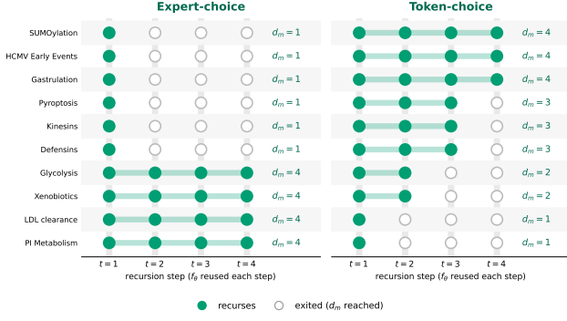
Figure 1: Two routing modes assign per-pathway depth d_m (real Prostate tokens; ● recurses, ○ exited; the block f_\theta is reused up to K=4 , so depth adds no parameters). Expert-choice fixes capacity per step; token-choice lets each pathway self-gate its depth.
