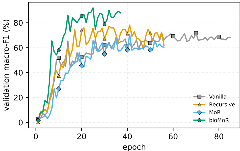
Baron: validation macro-F1 vs epoch
