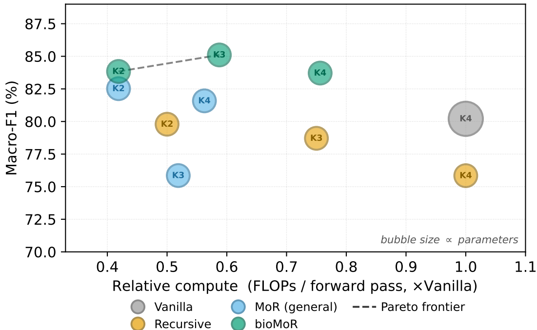
Accuracy vs. compute on Muraro (pancreas)
