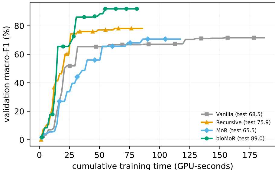
Baron: accuracy vs. training cost (learning curves)
