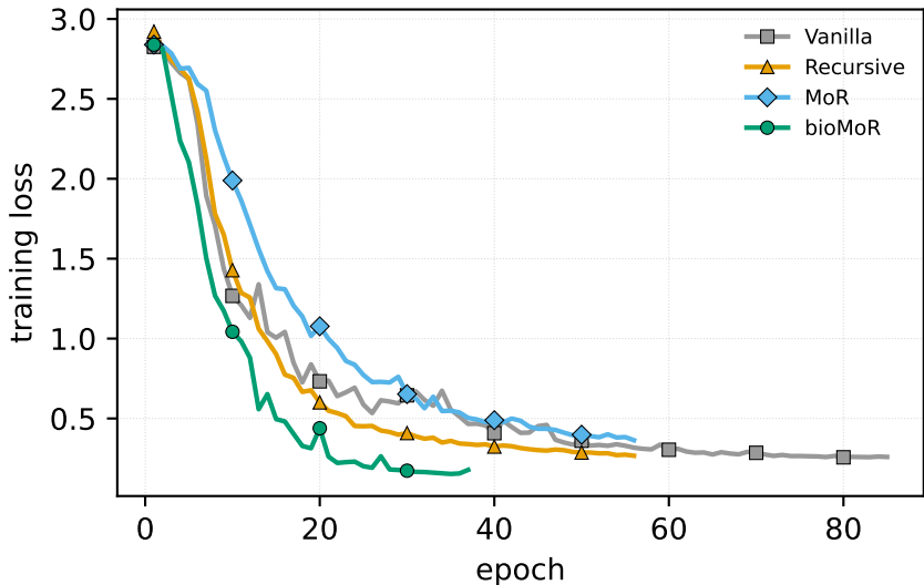
Baron: training loss vs epoch
