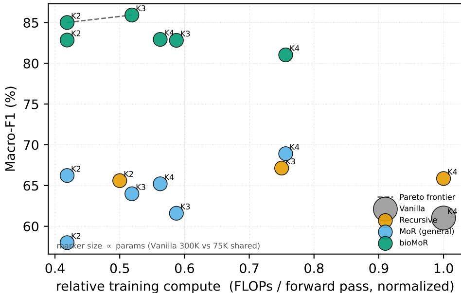
Baron: accuracy vs. compute (PROTOTYPE — FLOPs proxy)
