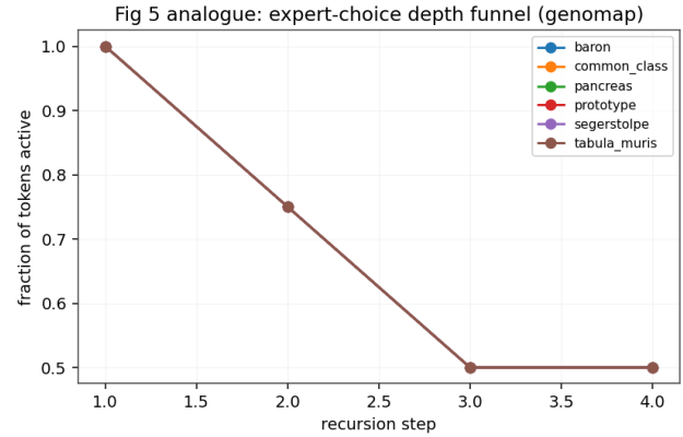
Figure 4: The expert-choice funnel: fraction of marker tokens still active at each recursion step.
