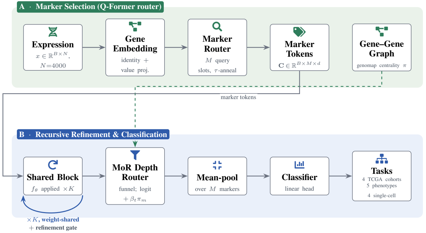
Figure 1: System overview. Panel A (marker selection): the expression vector is embedded gene-by-gene, then M learnable query slots cross-attend over all N genes (temperature annealed soft→peaked) to select interpretable marker tokens, a Q-Former-style router. Panel B (recursive refinement & classification): a single weight-shared block f_\theta is applied up to K times (loop-back arrow) with a per-marker refinement gate between passes; a Mixture-of-RecurSIONs router funnels capacity so each marker gets an adaptive depth d_m (deeply routed genes are candidate drivers). Biology-informed routing: a genomap gene-gene co-expression graph supplies a network-centrality prior \pi that is added (annealed by \beta_t ) to the depth-router logit (dashed arrow), so co-expression hub genes get a head start in the funnel without any label leakage. Tokens are mean-pooled and classified; the same pipeline serves all datasets, the four TCGA cohorts, five clinical phenotype tasks, and four single-cell cell-type datasets.
