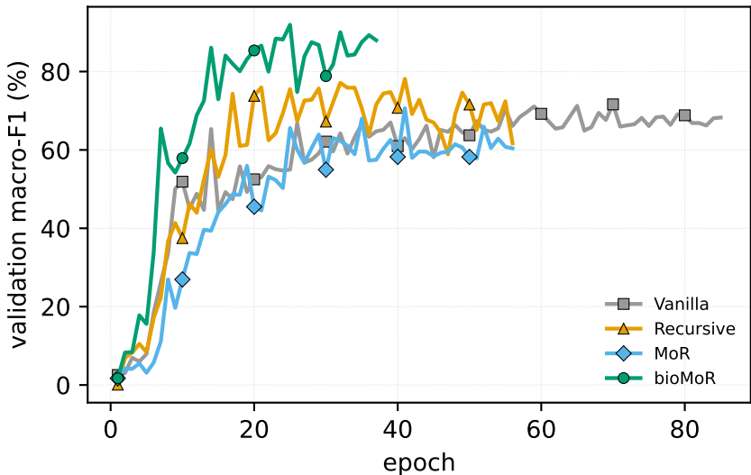
Baron: validation macro-F1 vs epoch
