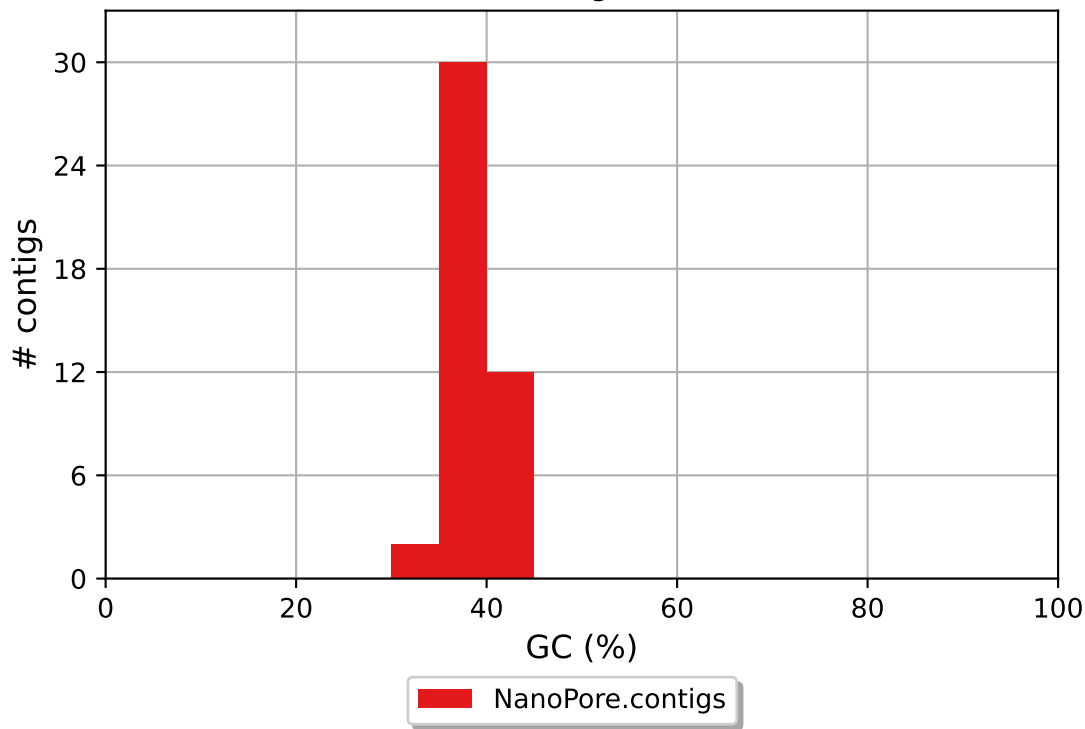
NanoPore.contigs GC content
