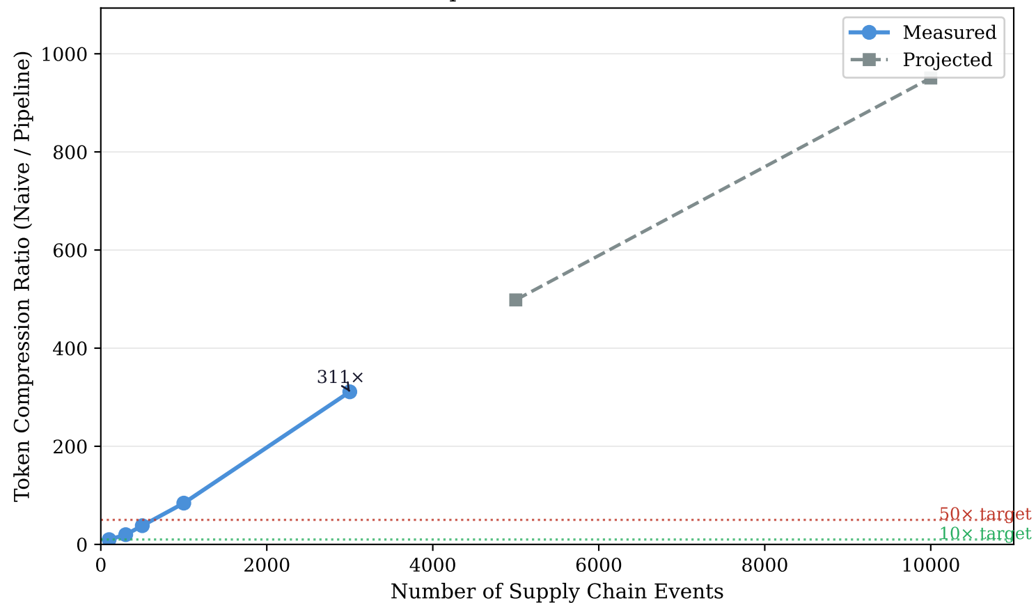
Token Compression Ratio vs. Event Scale
