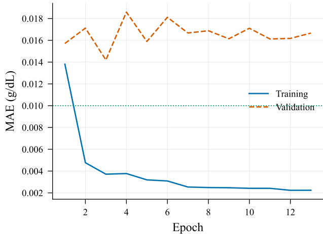
(b) Mean Absolute Error
