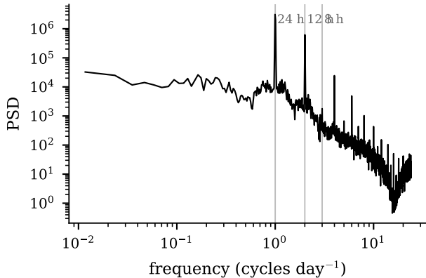
(b) GHI power spectrum
