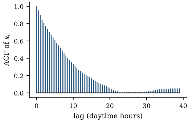
(a) clear-sky-index ACF
