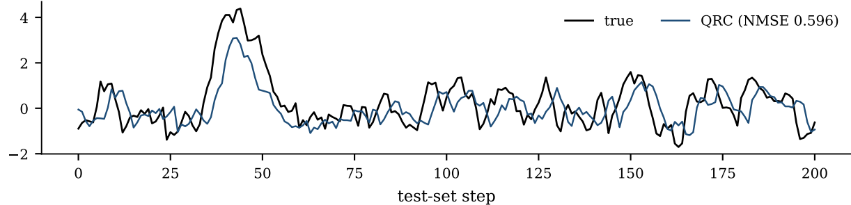
(c) ENSO SST anomaly, 3-month ahead (real data)
