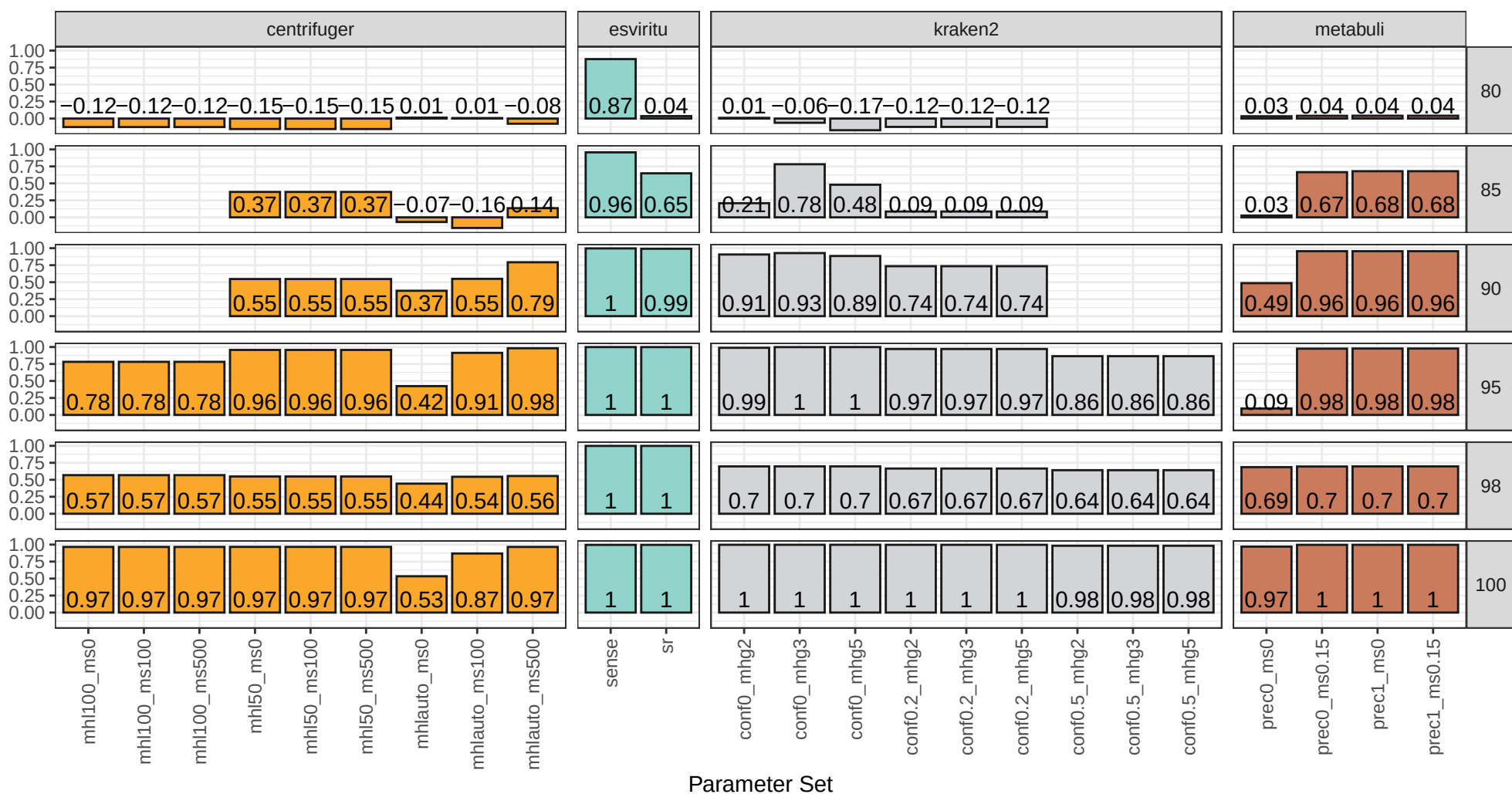
Pearson Correlation with Ground Truth
