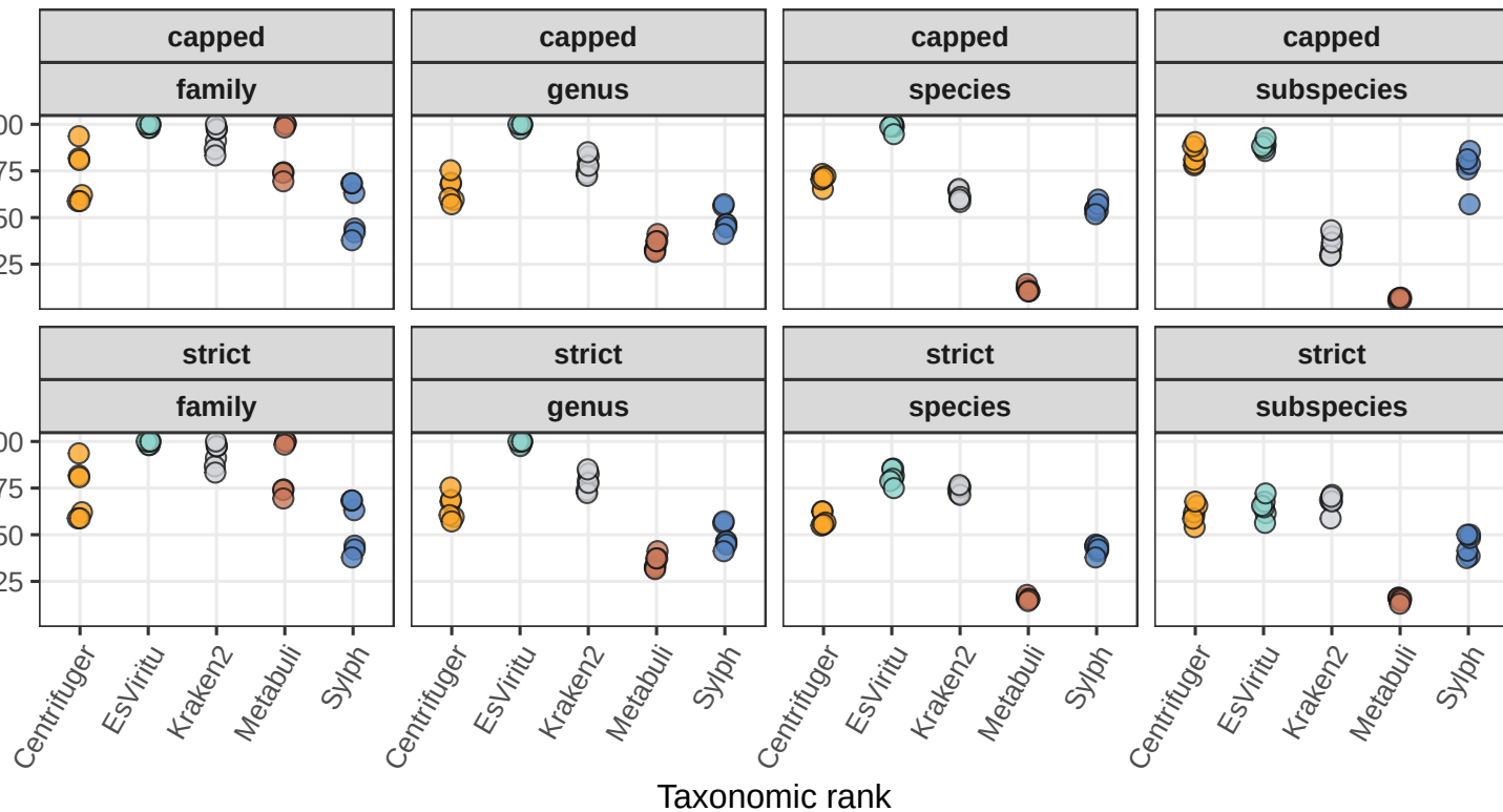
F1 Score: strict vs divergence-capped truth
