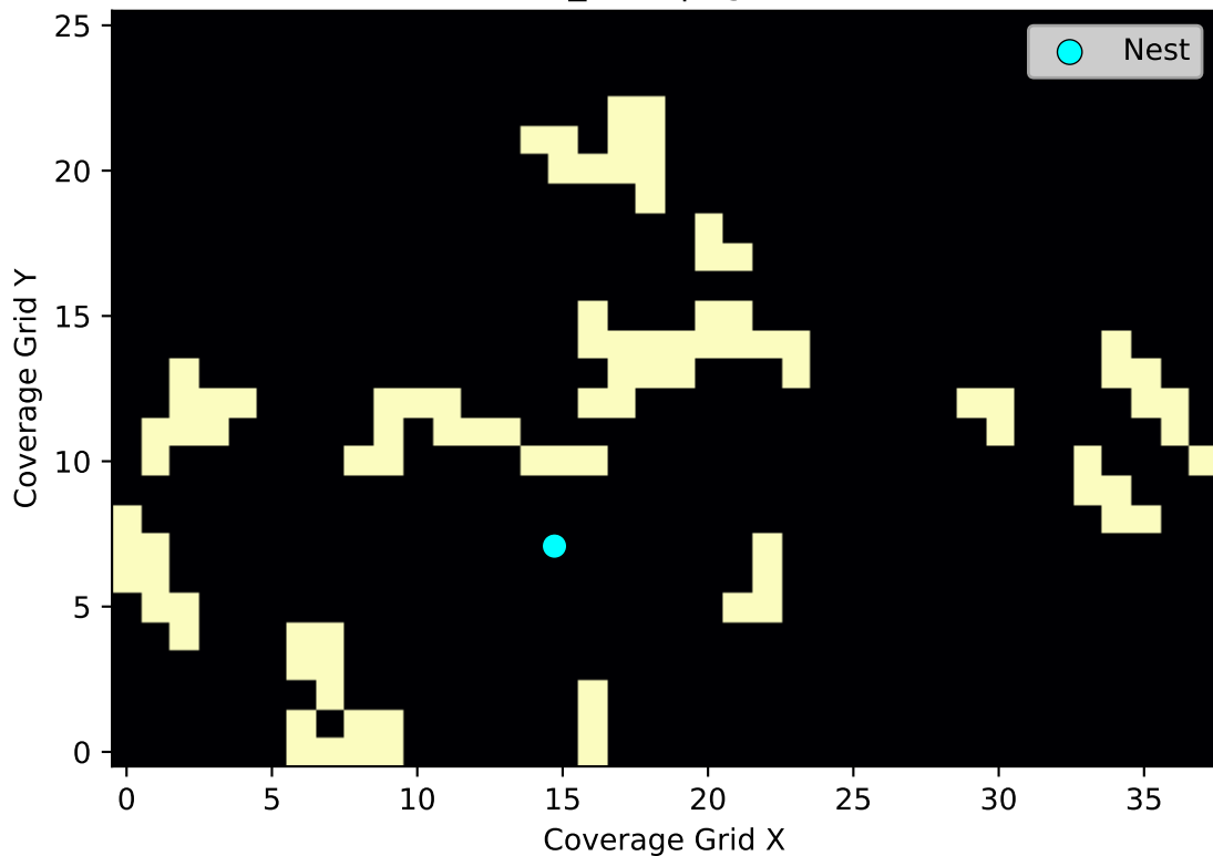
random_walk | agents=20
