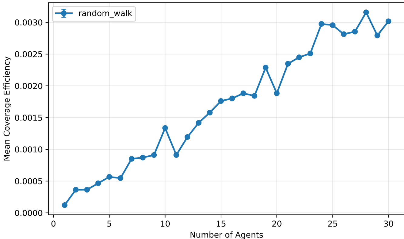
Coverage Efficiency vs Agents
