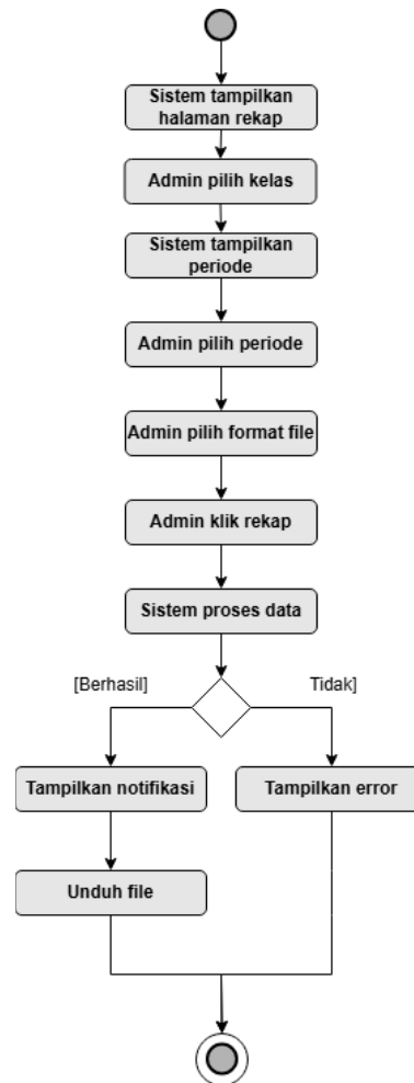
Gambar 3.14. Activity Diagram Rekap Absensi Siswa
