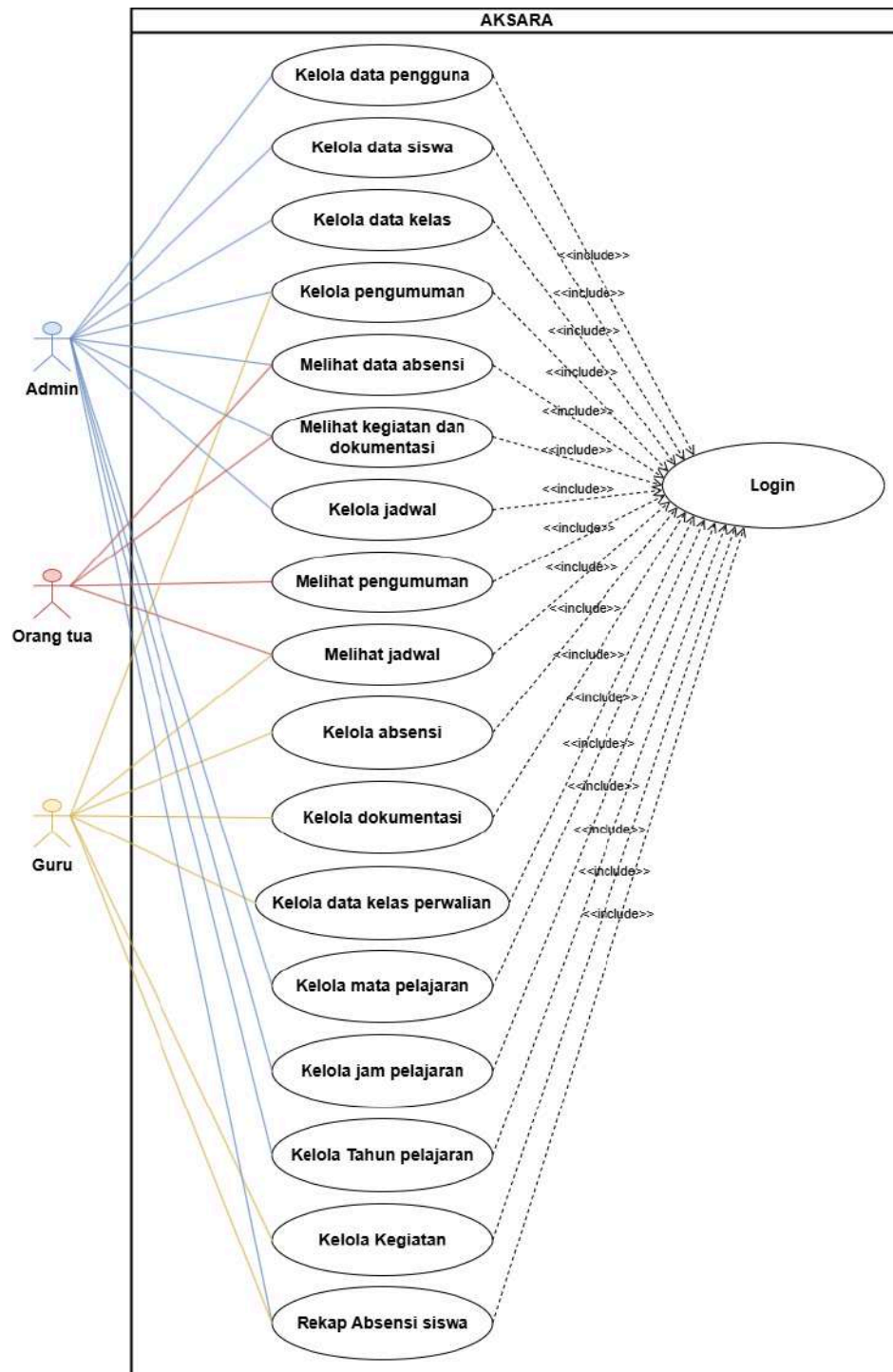
Gambar 3.2. Use Case Diagram
