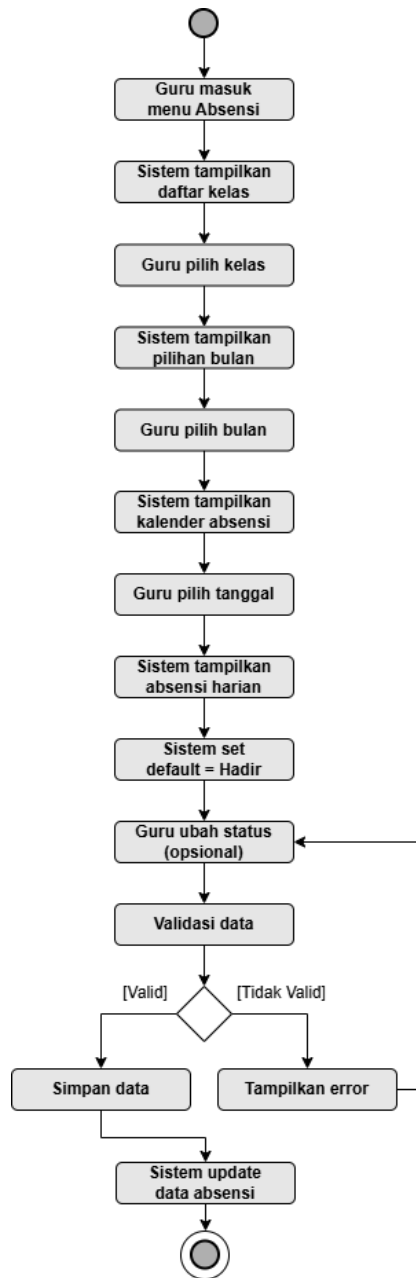
Gambar 3.21. Activity Diagram Kelola Absensi
