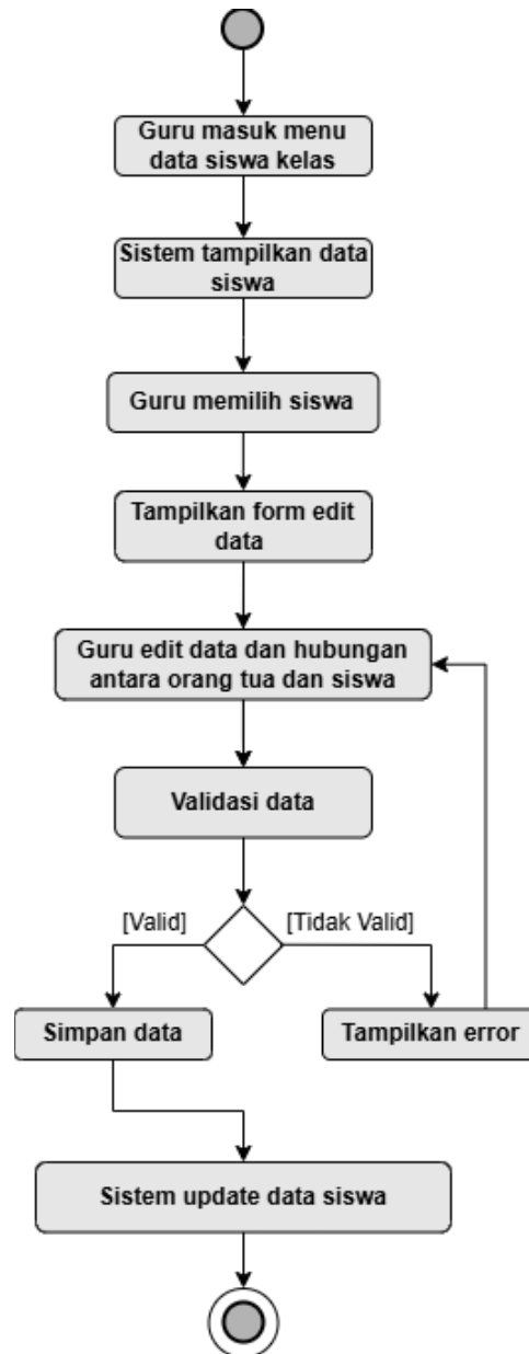
Gambar 3.24. Activity Diagram Kelola Data Kelas Perwalian
