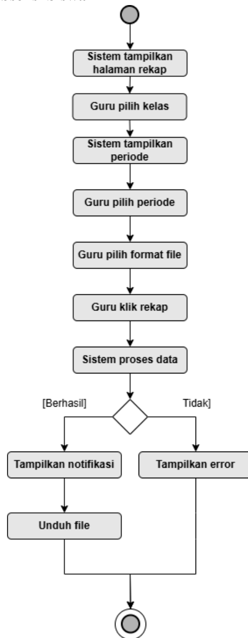
Gambar 3.25. Activity Diagram Rekap Absensi Siswa (Guru)
