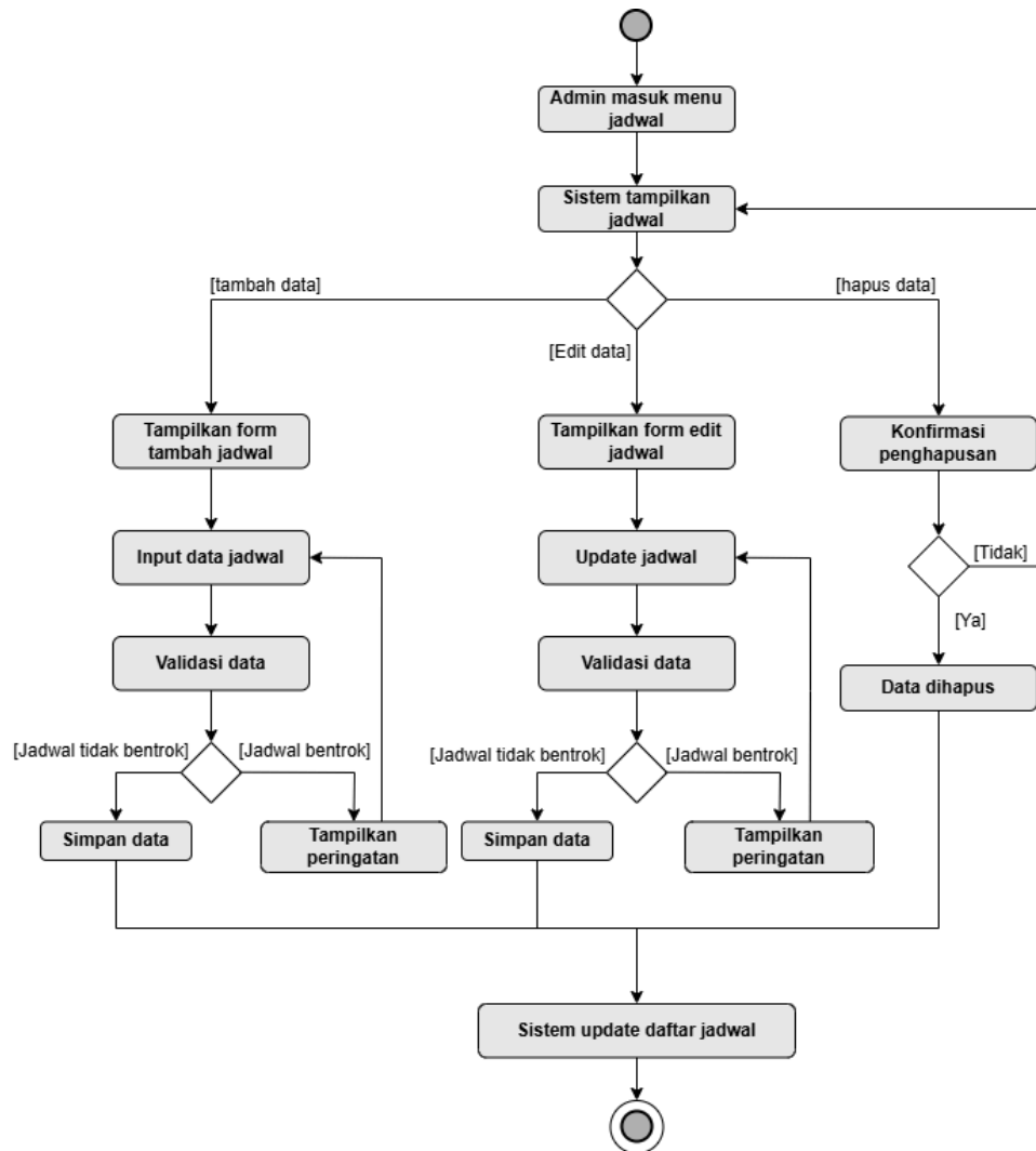
Gambar 3.10. Activity Diagram Kelola Jadwal
