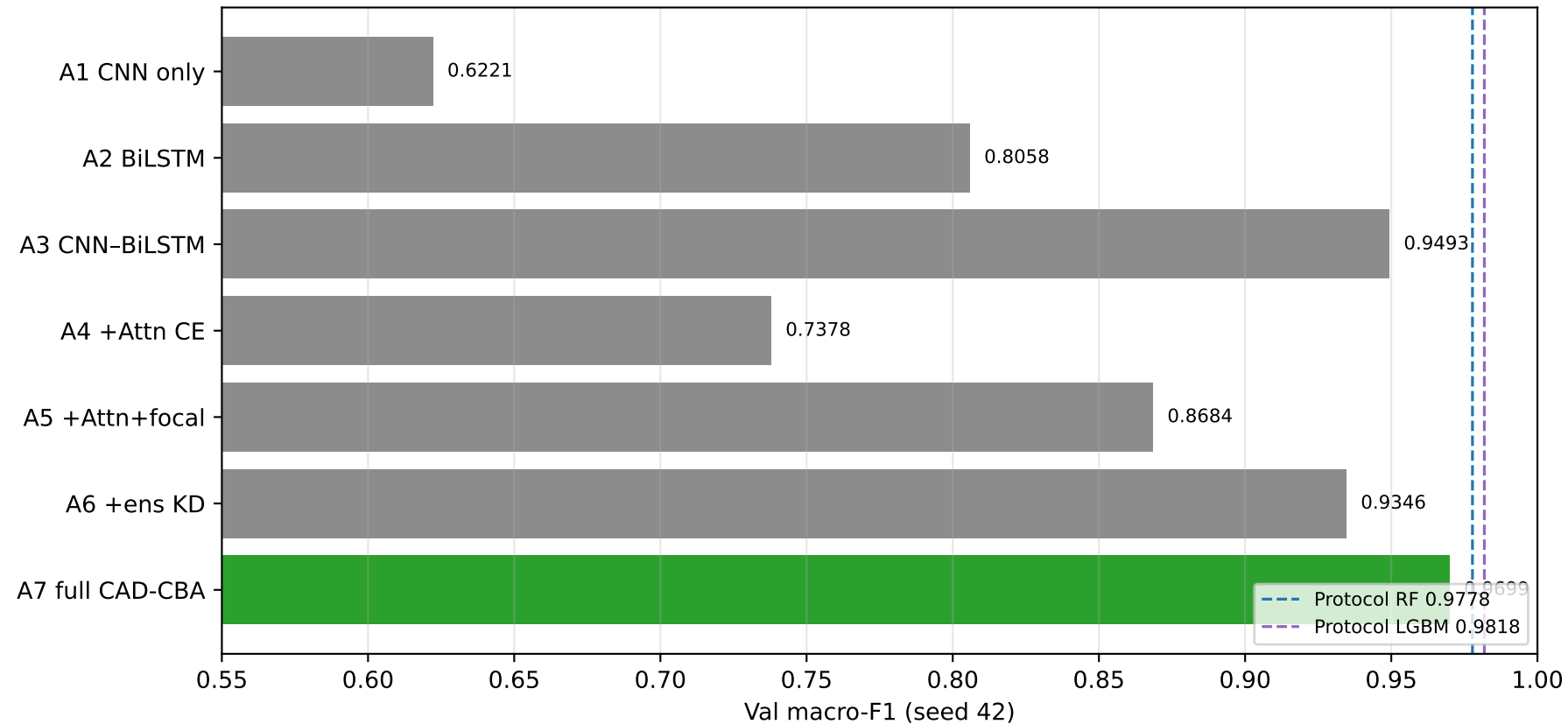
WP5a ablation ladder — package composition (not attention alone)
