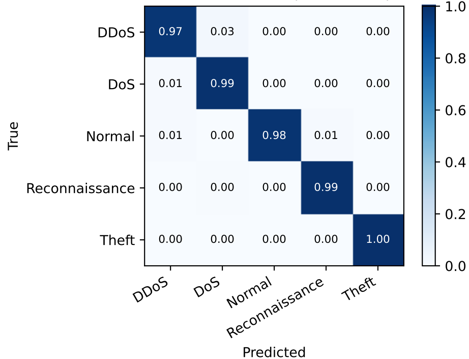
Row-normalized (recall view)
