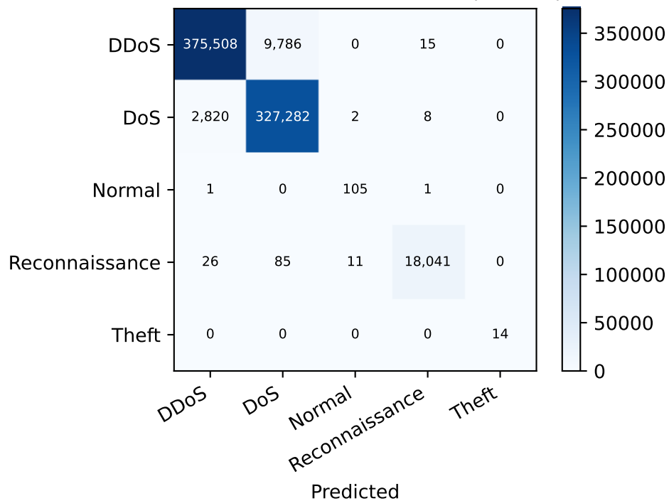
B14 seed42 TEST confusion (counts)
