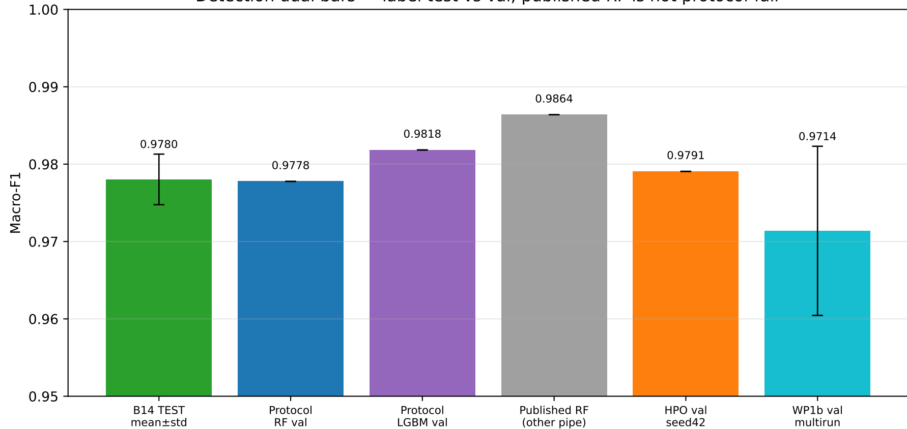
Detection dual bars — label test vs val; published RF is not protocol-fair
