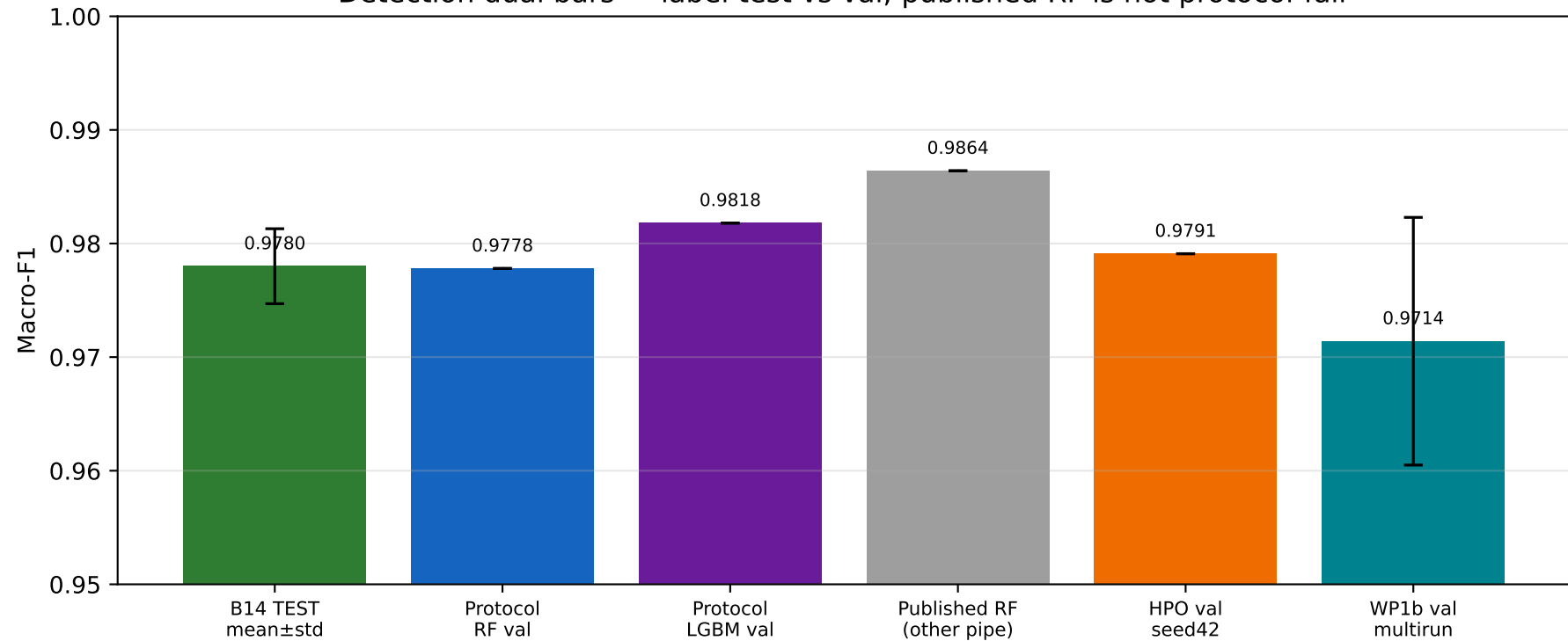
Detection dual bars — label test vs val; published RF is not protocol-fair
