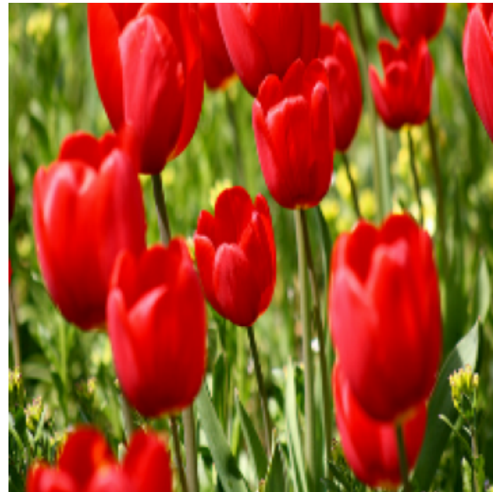
Adversarial Image
