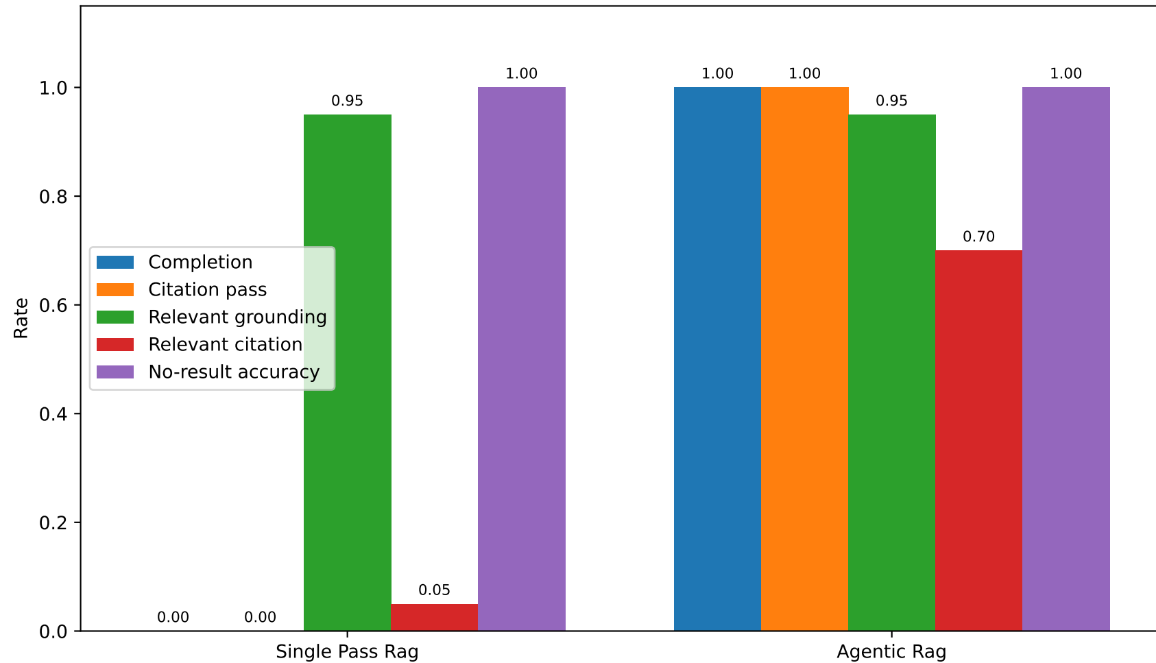
Single-Pass versus Agentic RAG
