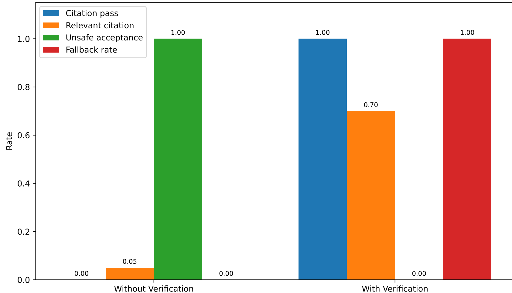
Verification-Stage Ablation
