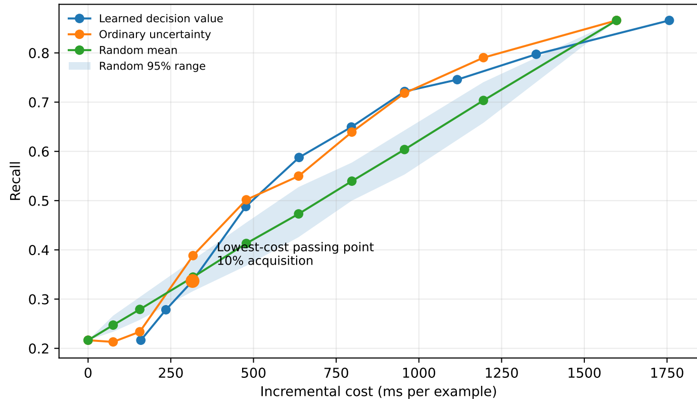
Development-only common-risk safety-cost frontier
