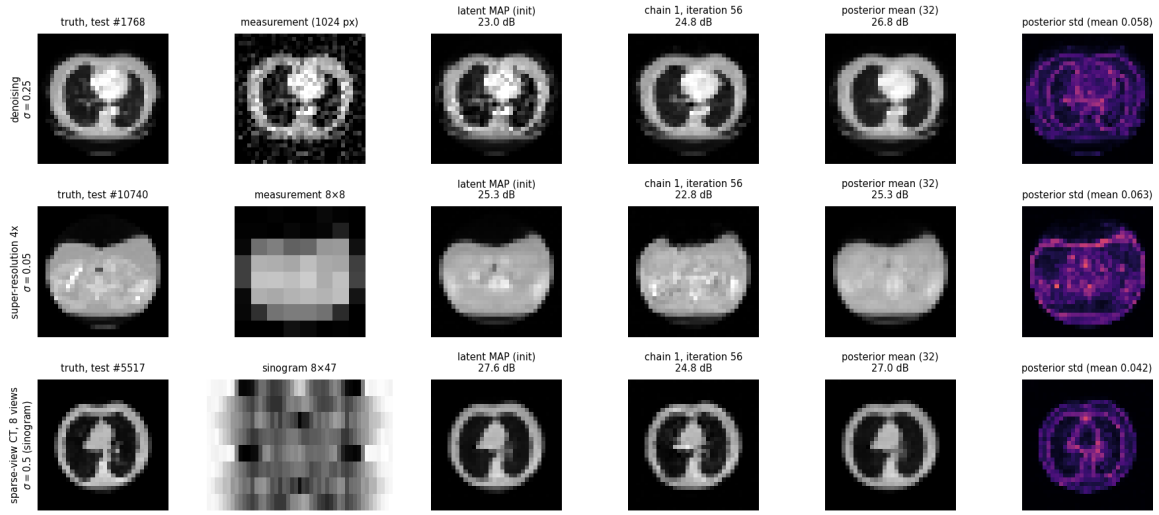
Figure 134: 32 px, one random walk per system ( L = 64 , 24 burn-in iterations, 32 recorded samples, from the latent MAP, with the diagonal mass matrix of the Methods): truth, measurement, the initial state, the last state, the mean and std of the 32 samples. The 32 samples are the frames of langevin_32_walk_{denoise,sr_4x,ct}.mp4 .
