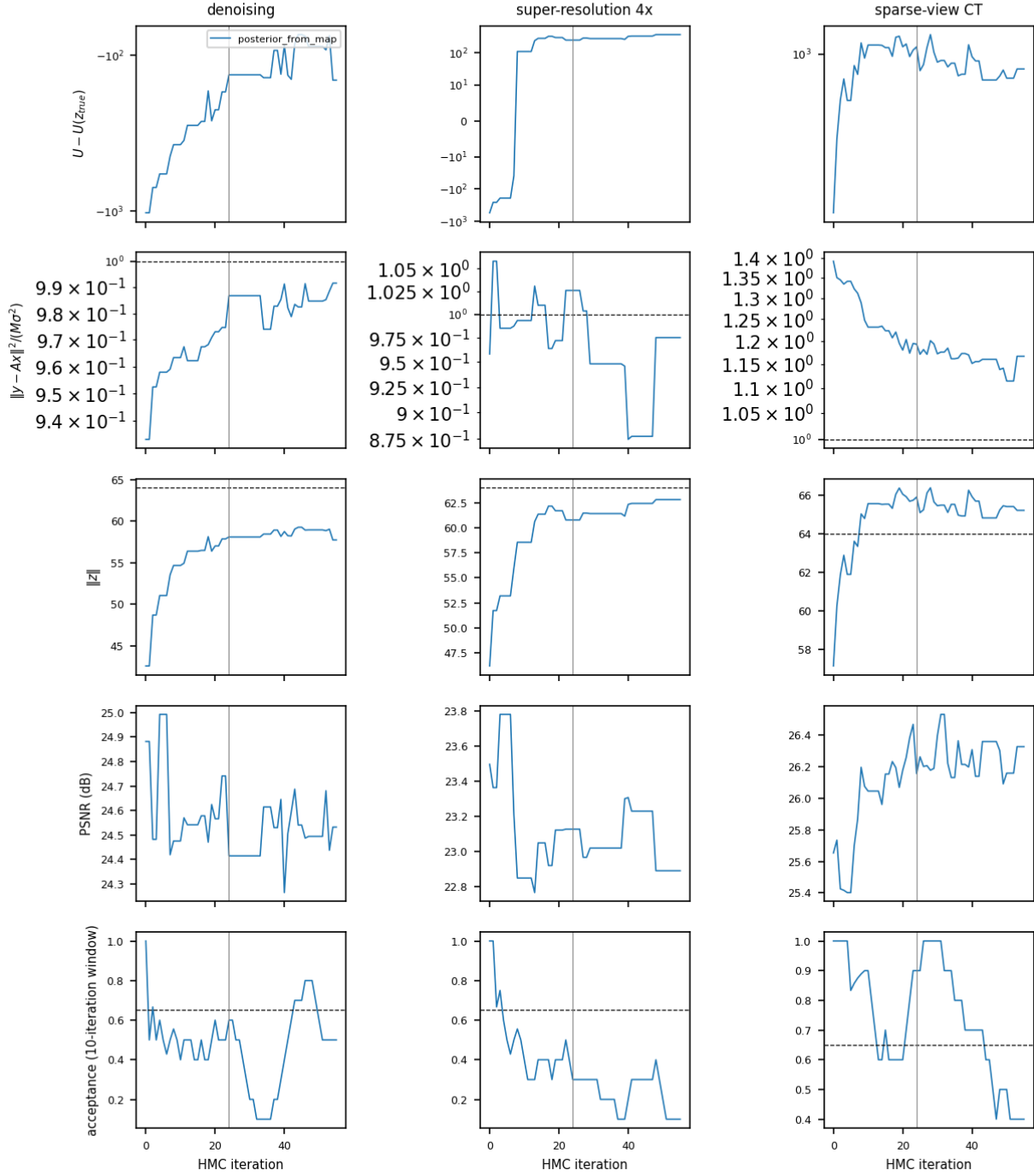
Figure 137: 64 px, traces of the random walks.
