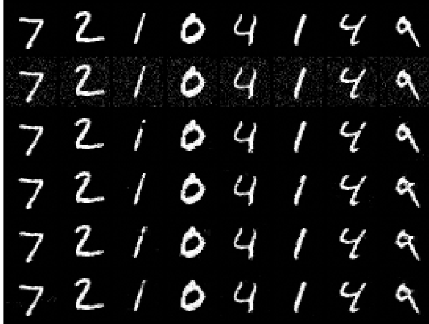
Figure 70: denoise . Rows: ground truth; pseudo-inverse A^+y ; three posterior samples f^{-1}(z) , z \sim \mathcal{N}(A^+y, \Sigma_1) ; posterior mean over 8 draws. Display is clamped to [-1, 1] : \sigma = 0.2 is 10% of the intensity range, and the noise row looks milder than that because the negative half of the background noise is below the black level.
