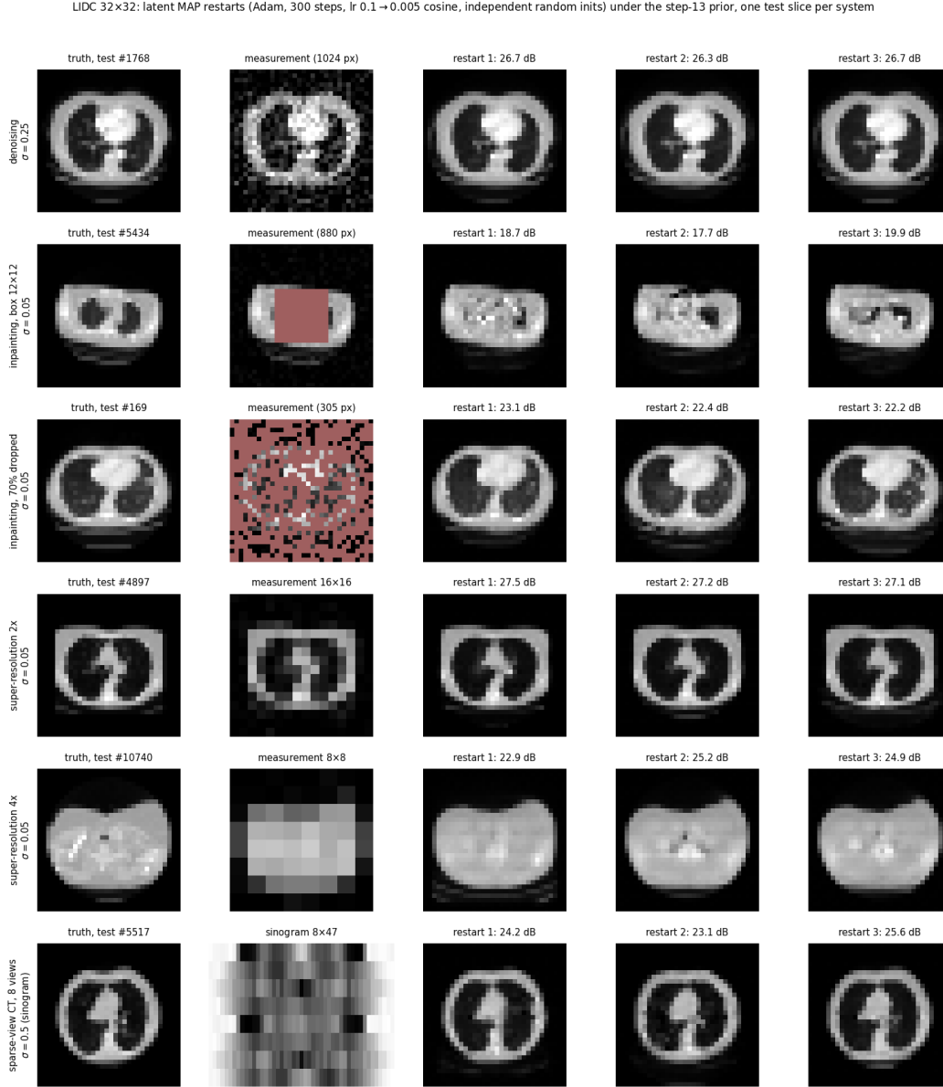
Figure 113: 32 px: truth, measurement (masked pixels in red; the low-resolution image; the 8 \times 47 sinogram) and three latent-MAP restarts with their PSNR, one test slice per system.
