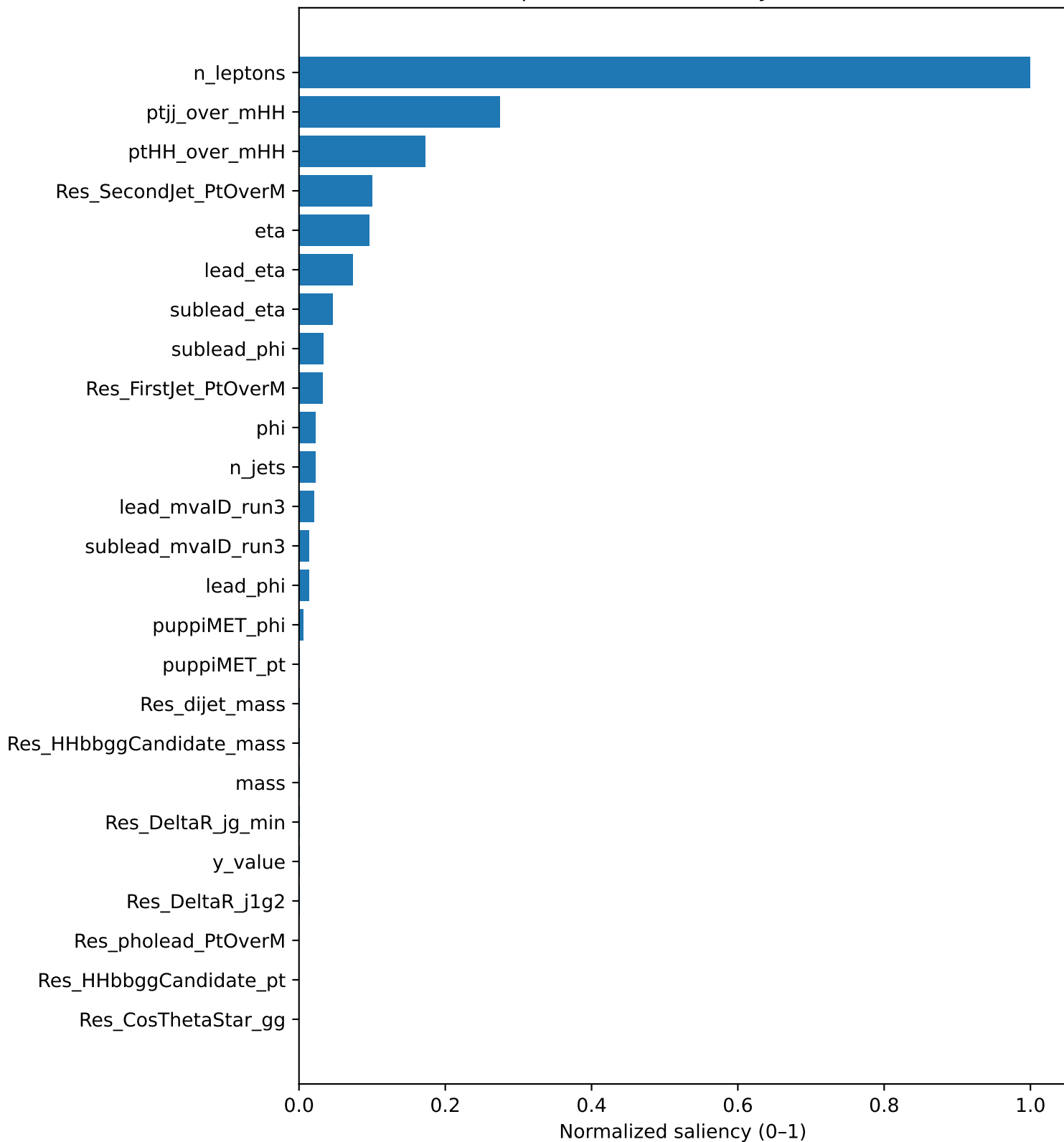
Input-Gradient Saliency — TEST
