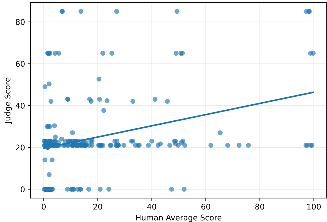
Qwen2.5-7B Judge Pearson r = 0.340
