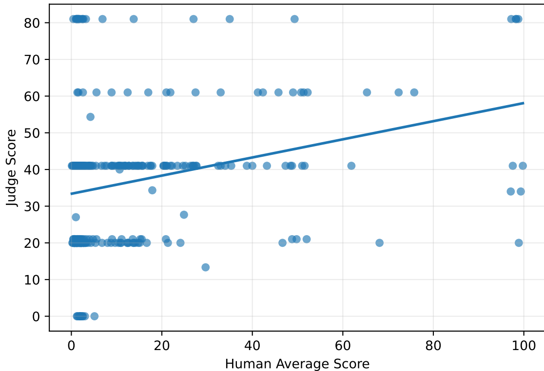
LLaMA-3-8B Judge Pearson r = 0.275
