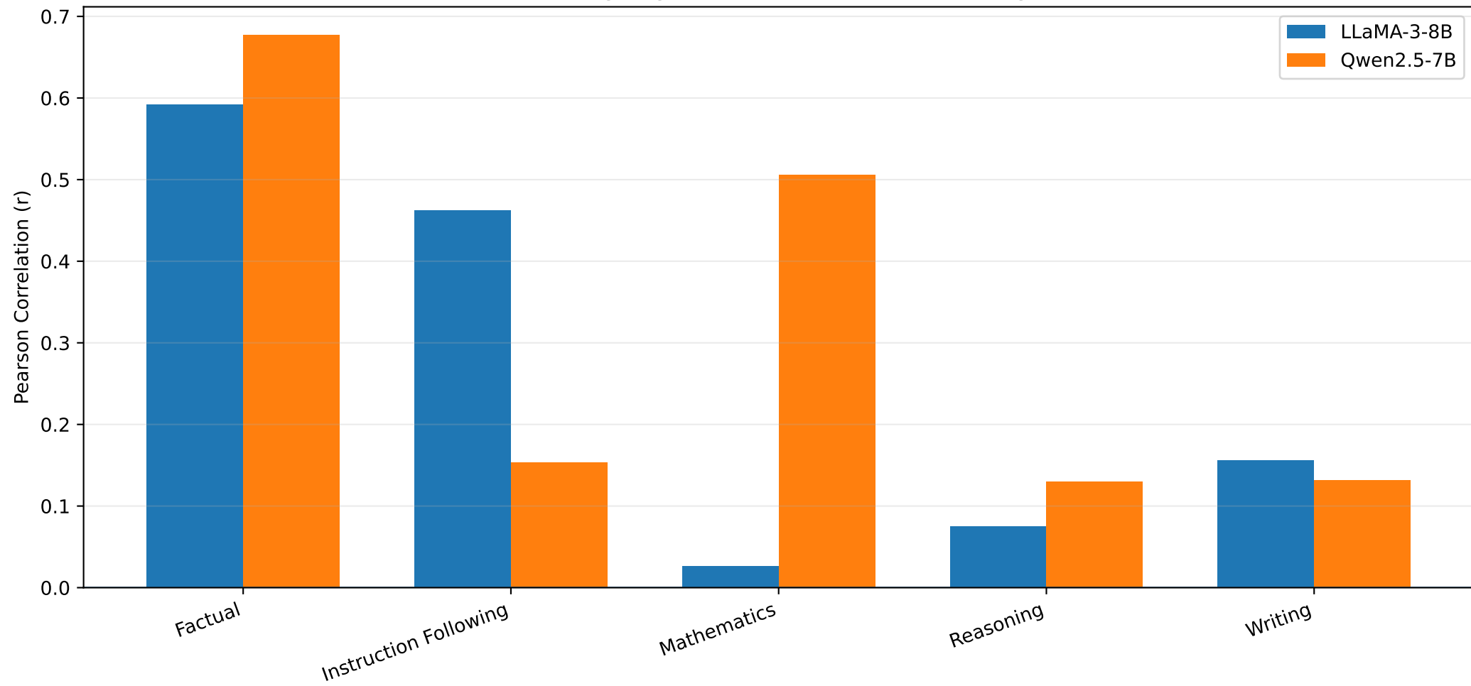
Human-Judge Agreement Across Question Categories
