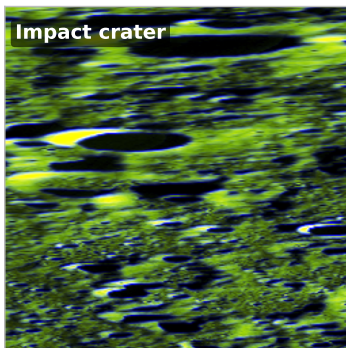
Real tile
