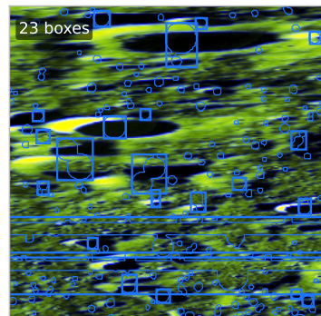
Instance boxes
