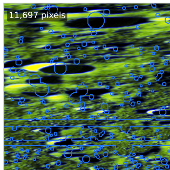
Semantic mask
